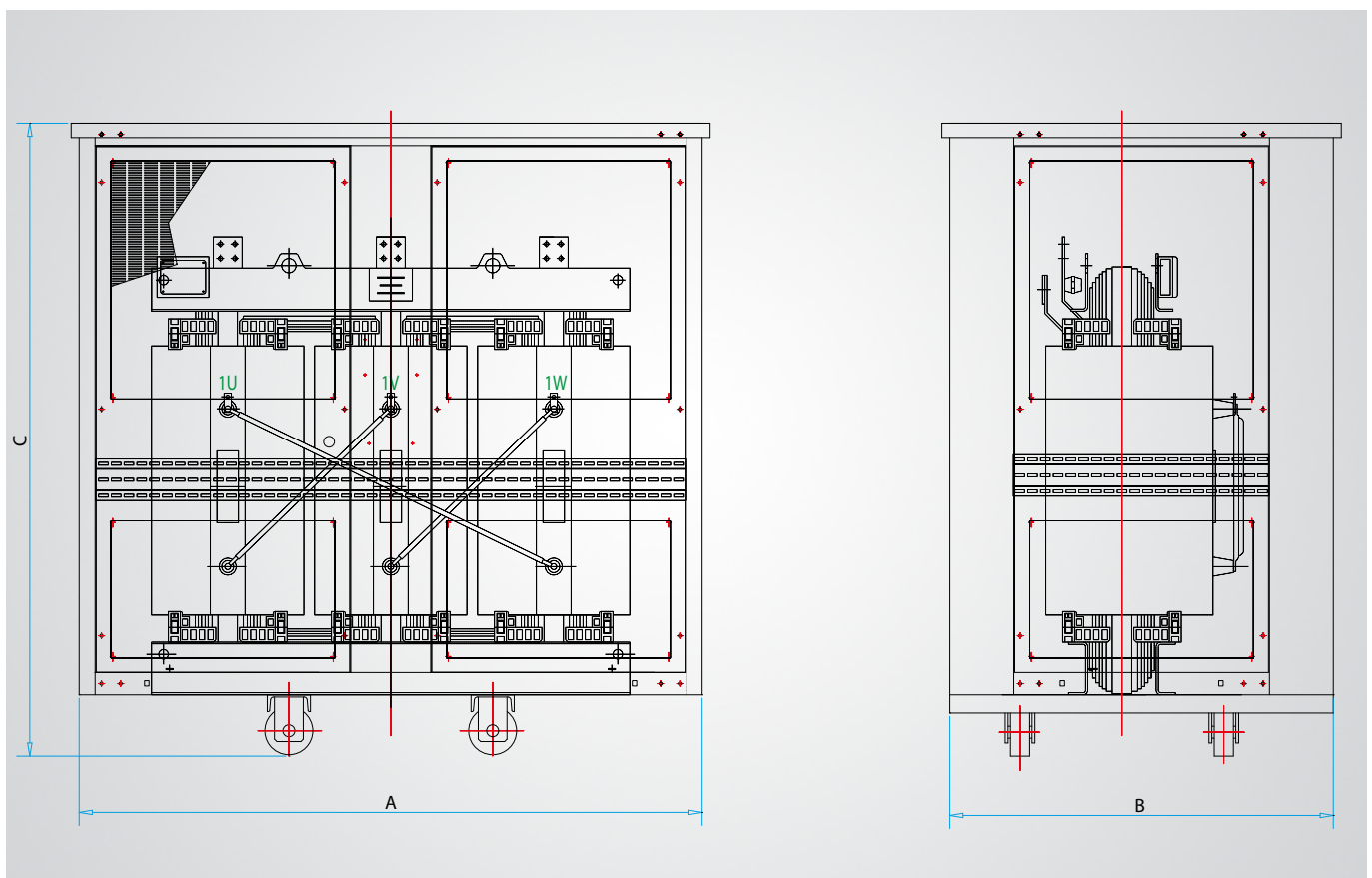
Metal Enclosure Drawing
