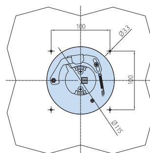
Extended Rotary Handle
