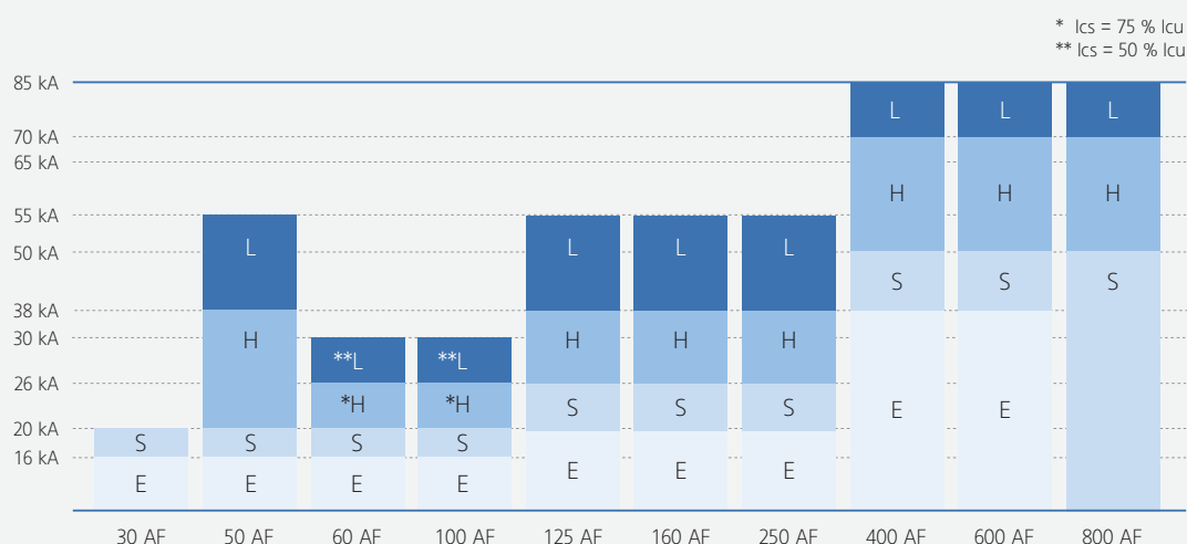
Rated Short-Circuit Current by AF, (Ics = 100 % Icu, at 440/460 V)
